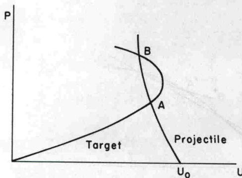
FIG. 7. Impedance match solution for impact of a projectile with a target whose Hugoniot contains a region for which (dP/du)_H < 0 . States A and B satisfy interface conditions.
